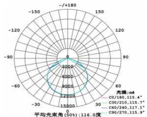
Lighting Distribution Diagram:
